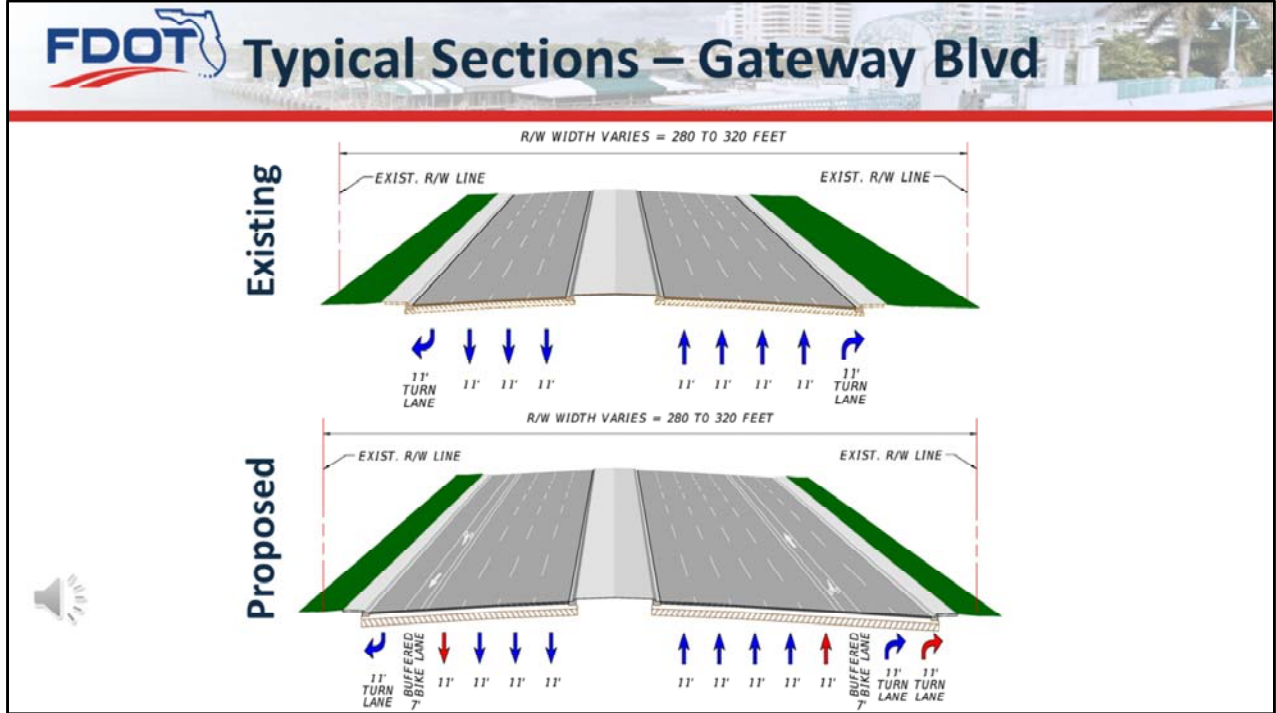
The existing and proposed roadway typical sections for Gateway Blvd are shown here.
