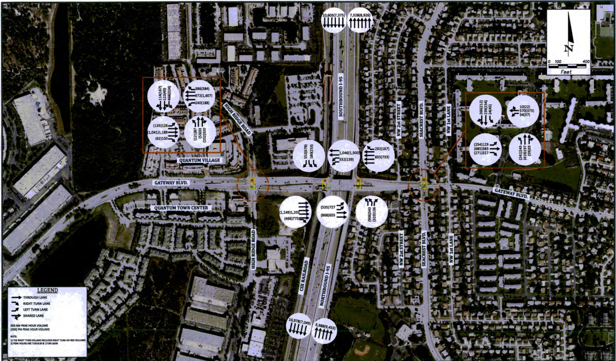
Figure A3: Existing (2015) Balanced Intersection Turning Movement Volumes I-95 at Gateway Boulevard Interchange PD&E Study for I-95 at Boynton Beach Boulevard and Gateway Boulevard Interchanges
